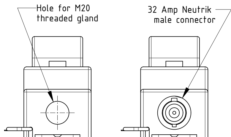
SUPPLY CONNECTION OPTIONS
